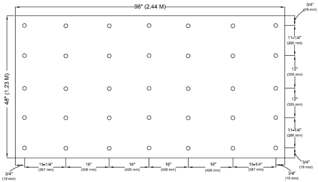
Diagram 2 – Standard Fastening Pattern for Horizontal Installation:
